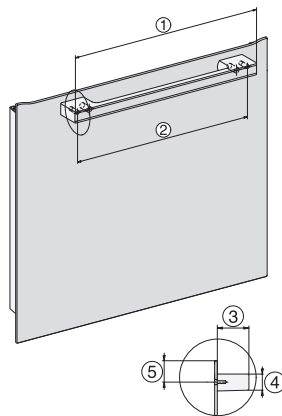
H2860-55B/BP, installation drawing
