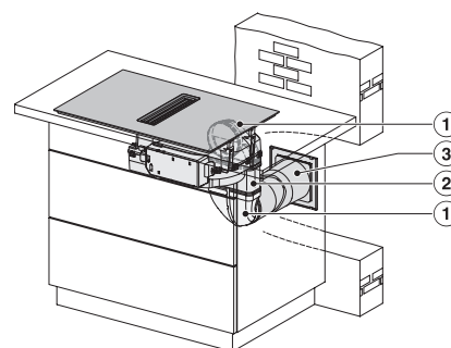
KMDA7676FL, KMDA7876FL – Installation variant 2 Basis – drawing
